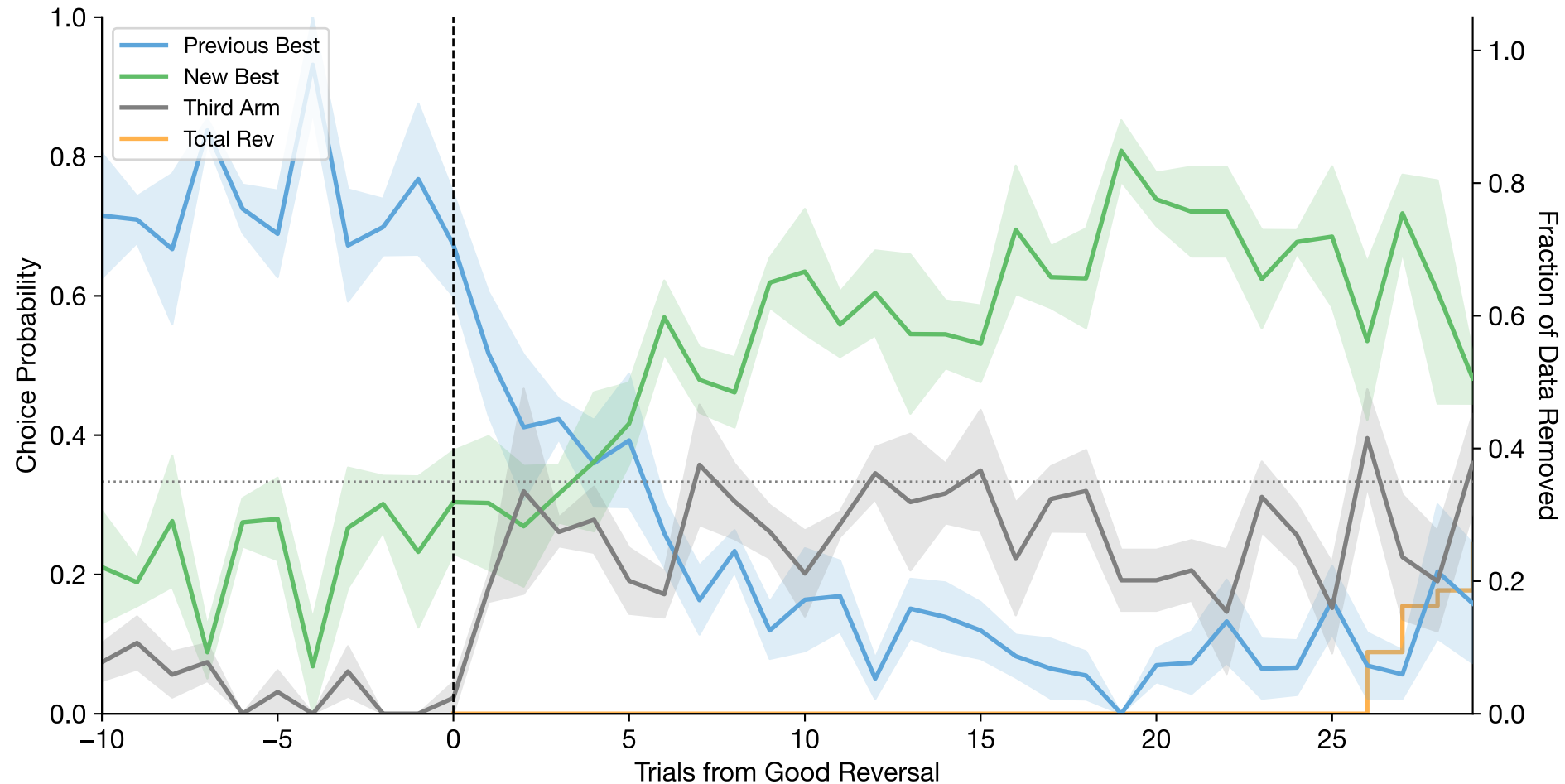
Good Reversal-Aligned Choices (mean \pm se across subjects | n=4 subjects, n=43 reversals)
